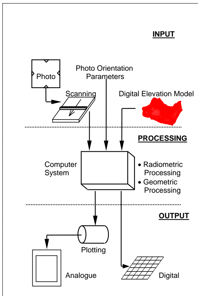
Figure 3: Process of Digital Orthophoto Production
