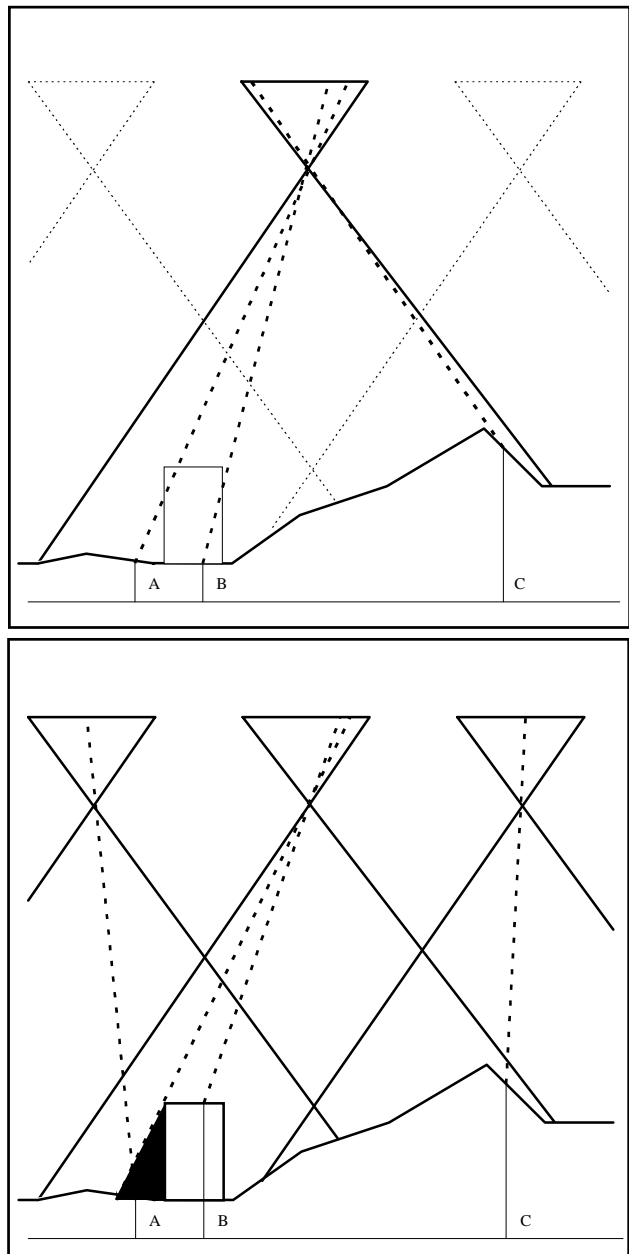
Figure 5: Properties of True Orthophoto
