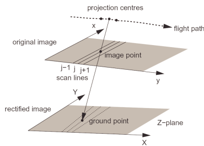
Figure 6. Direct method for image rectification
